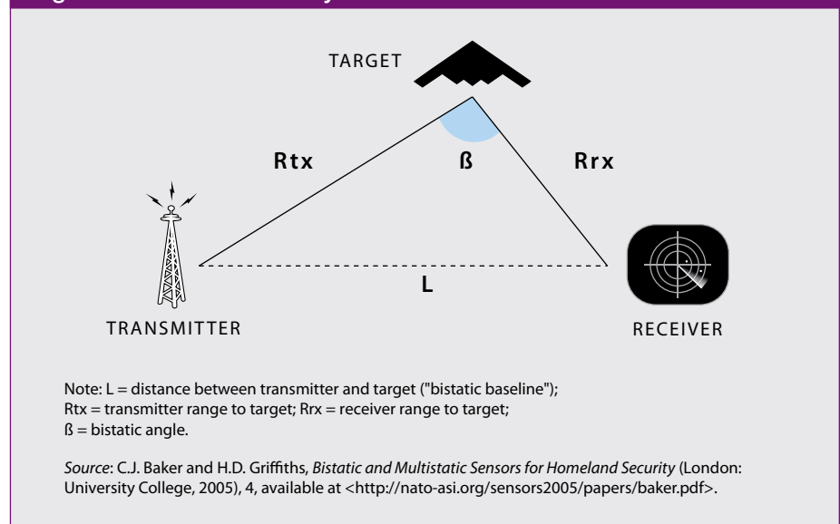
Figure 1. Bistatic Geometry
